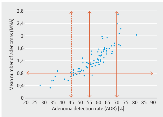
► Fig. 1 Correlation between adenoma detection rate and mean number of adenomas per colonoscopy.
