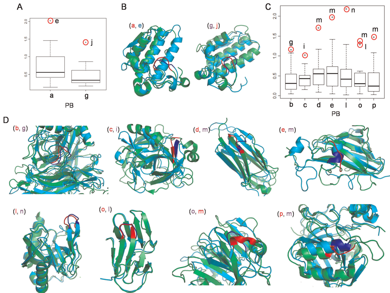
Figure 7. PB substitutions highly preferred in certain SCOP classes. The cases where the class-specific substitution scores associated with each PB (each row in the substitution matrix) has a correlation less than 0.95 when compared to the global matrix, were looked into. The absolute differences (class specific vs Global) of substitution patterns (respective rows) were plotted as a boxplot, to identify outliers. Substitution scores lying outside a 1.5 inter-quartile range (IQR), were considered as outliers or significantly different from the global substitutions. For the all- \alpha class, (A) the plots are generated for PBs a and g . (B) highlights examples of backbone conformations corresponding to substitutions detected as outliers. Similarly, boxplots were generated for the all- \beta class (C) and the examples of significantly different substitutions are shown (D). doi:10.1371/journal.pone.0038805.g007
