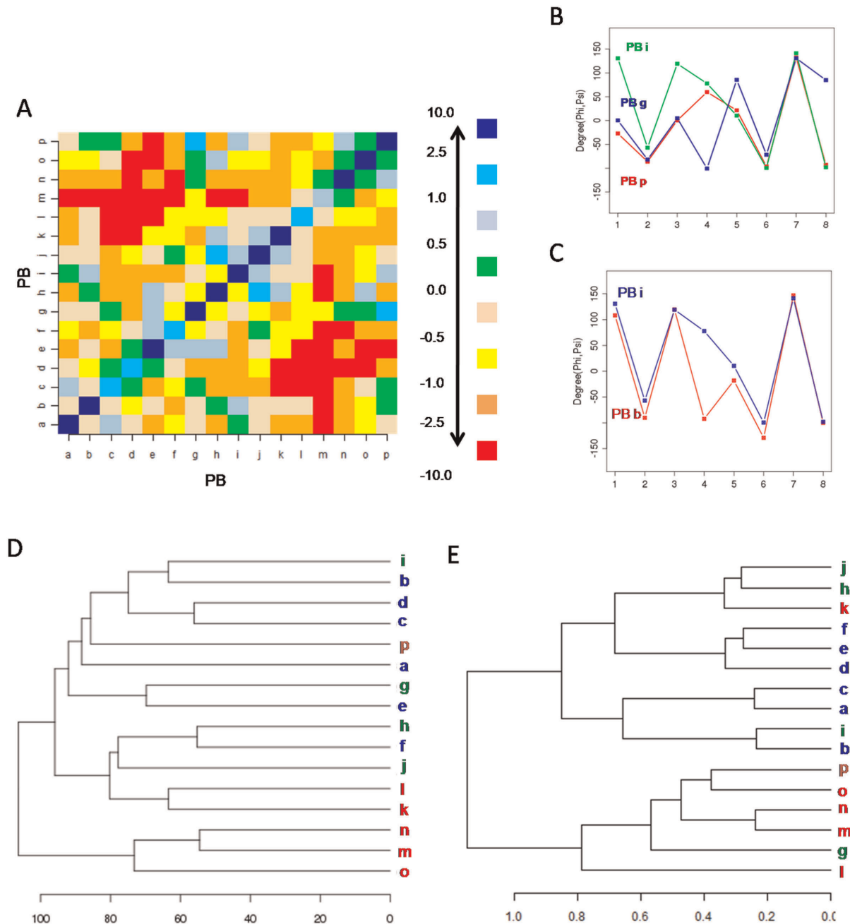
Figure 3. PB substitutions. (A) The variation in substitution score in the PB substitution matrix is highlighted using a colour-code, as shown. (B) The series of dihedral angles ( \psi_{i-2}, \phi_{i-1}, \psi_{i-1}, \phi_i, \psi_i, \phi_{i+1}, \psi_{i+1}, \phi_{i+2} ), associated with the PB substitutions ( p, g ) and ( p, i ) and (C) ( b, i ). These represent some of the preferred local conformational changes (D) Hierarchical clustering of PBs based on the similarity of dihedral angles, measured in terms of angular rmsd . The PBs frequently associated with helices are in red, those found often with beta strands are in blue and the rest are in green (E) Clustering of PBs based on the substitution pattern associated with each PB (see Methods ). doi:10.1371/journal.pone.0038805.g003
