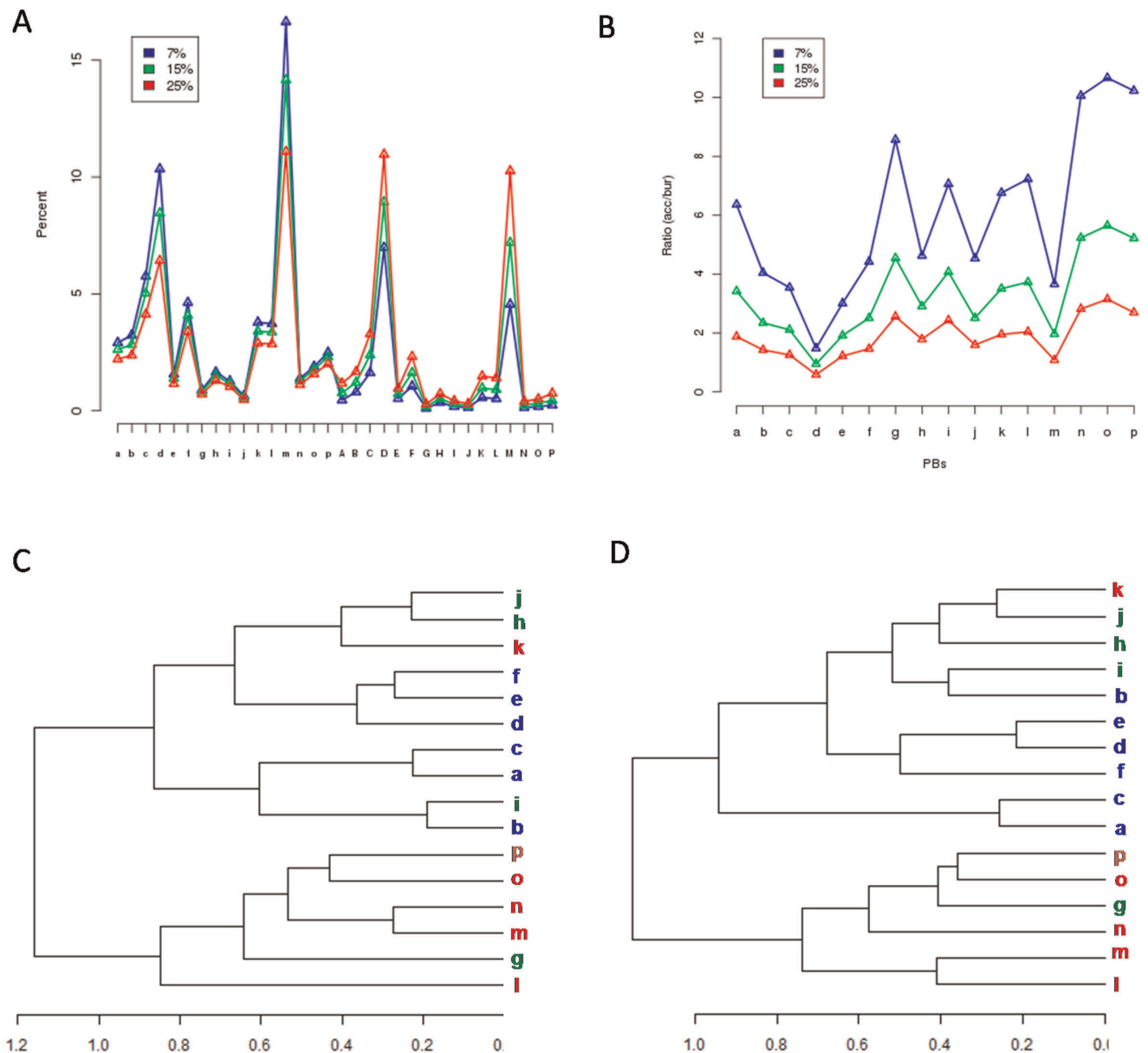
Figure 4. Clustering PBs based on substitution patterns. (A) Distribution of accessible and buried PBs classified based on different accessibility cut-offs of 7%,15% and 25%. Ratio of frequency of exposed PBs to that of buried, plotted for each of the 16 PBs (B) Hierarchical clustering of PBs classified as exposed (C) and buried (D) at an accessibility cut-off of 15%. The clustering is based on the correlation of substitution scores. doi:10.1371/journal.pone.0038805.g004
