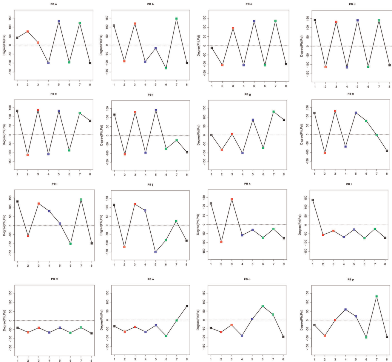
Figure 1. PBs series of \phi, \psi backbone dihedral angles. For each PB the series of 8 dihedral angles ( \psi_{1-2} , \phi_{1-1}, \psi_{1-1} , \phi_i, \psi_i , \phi_{i+1}, \psi_{i+1} , \phi_{i+2} ), numbered from 1 to 8, are plotted. i indicates the position of an amino acid in the protein. doi:10.1371/journal.pone.0038805.g001
