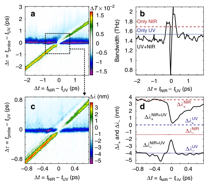
Figure 3 | Two-colour pumping effects. (a) Change in the probe pulse transmission as a function of the pump-probe delay ( \Delta\tau ) and the inter-pump delay ( \Delta t ). The ultraviolet (UV) pump decreases the transmission, whereas the NIR increases it. The combined effect produces a \Delta t -dependent modulation. The modulation bandwidth is evaluated by performing a Fourier transform along \Delta\tau , and is shown by the black curve in (b). For delays close to \Delta t = 0 , the modulation bandwidth can be decreased or increased by the two-colour combined effect. The blue and red dashed lines show the bandwidth of the ultraviolet-only and NIR-only driven modulation. (c) Measured central wavelength shift of the transmitted probe pulse ( \approx 15 \text{ nm} bandwidth) in a zoomed \Delta t - \Delta\tau region (square box in (a)). The ultraviolet pump blue shifts the probe wavelength, whereas the NIR pump does the opposite. At \Delta t \approx 0 , the opposite effects almost entirely cancel the wavelength shift. (d) Summary of the findings in (c), showing the maximum positive ( \Delta\lambda_+ ) and negative ( \Delta\lambda_- ) wavelength shift for the NIR-only (red dashed/dotted), ultraviolet-only (blue dashed/dotted) and two-colour (solid black) AZO excitation.
