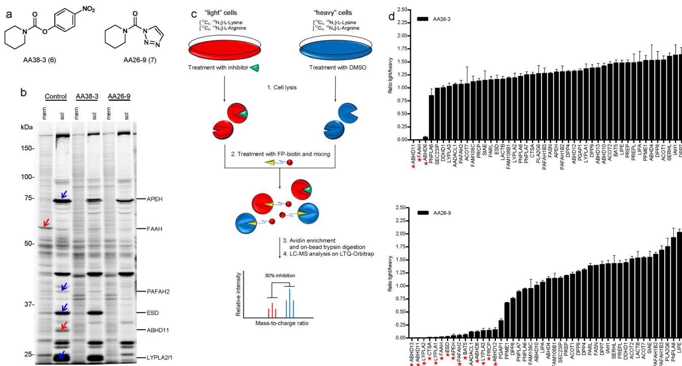
Figure 2. Comparative ABPP of piperidine-based carbamate (AA38-3) and triazole urea (AA26-9) inhibitors. (a) Structures of AA38-3 and AA26-9. (b) Competitive ABPP of AA38-3 and AA26-9 in BW5147-derived murine T-cell hybridoma cells. Cells were cultured with 20 \mu\text{M} inhibitor or DMSO as a control for 4 h, lysed, separated into soluble and analyzed by competitive gel-based ABPP. Blue and red arrows mark SHs that were inhibited by AA26-9 and both AA26-9 and AA38-3, respectively. (c) Schematic representation of a competitive ABPP-SILAC experiment. Isotopically "light" (red) and "heavy" (blue) mouse T-cells are treated with inhibitor and DMSO, respectively, for 4 h. Cells are lysed, proteomes are treated with FP-biotin, and combined in a 1:1 ratio. Biotinylated proteins are enriched, trypsinized, and analyzed by LC-MS/MS. SH activities are quantified by comparing intensities of light and heavy peptide peaks. (d) Identification of SH targets for AA38-3 (top) and AA26-9 (bottom) in mouse T-cells by ABPP-SILAC. Cells were cultured with inhibitor (20 \mu\text{M} ) or DMSO as a control for 4 h prior to analysis by competitive ABPP-SILAC. Asterisks mark SHs that were inhibited by > 75\% . Bars represent the means \pm s.e.m of light/heavy-ratios of identified tryptic peptides in both soluble and membrane proteomes for two independent biological replicates.
