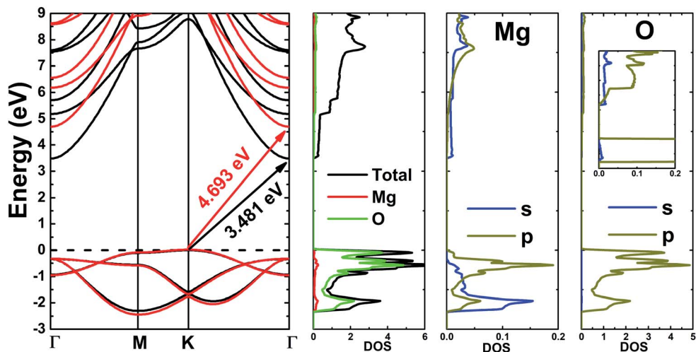
Fig. 3 Band structure (black lines and red lines represent the results from the PBE and HSE06 functionals, respectively), and total and partial density of states (states per eV) of the pristine MgO monolayer.
