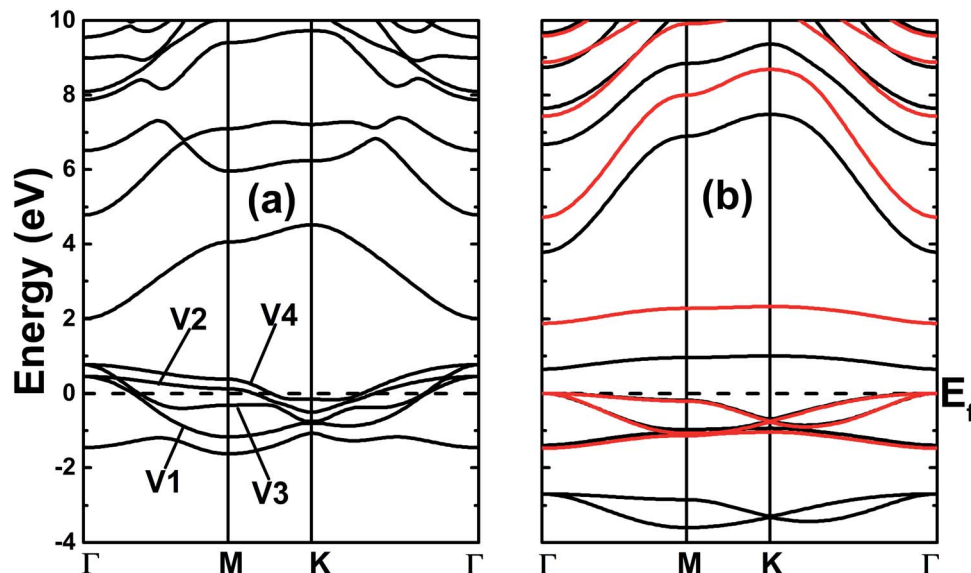
Fig. 6 Band structures of the (a) N- and (b) F-functionalized MgO monolayers (black lines and red lines represent the results obtained with the PBE and HSE06 functionals, respectively).
