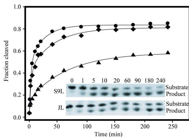
Figure 3 Kinetic analysis of hairpin-ribozyme constructs used in this study. Substrate-cleavage reactions were carried out under single-turnover conditions. For each construct (circles, S9-linked; diamonds, C3-linked; triangles, junctionless, JL) time courses were fitted to a double-exponential kinetic equation (see §2.4). Inset: representative gel images of the cleavage time course for the S9 and JL constructs; similar results were observed for the C3 construct (data not shown). Bands represent 5'-Cy5-labeled 13-mer substrate and 8-mer product strands.
