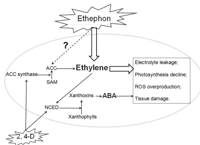
Figure 5. The difference in modes of action between ethephon and 2, 4-D. 2, 4-D induces the production of ACC synthase, therefore catalyzes the synthesis of ACC. ACC is the precursor of ethylene and can be converted into ethylene under catalysis by ACC oxidase. 2, 4-D also induces the production of NCED, which catalyzes the pyrolysis of xanthophylls to form xanthoxin, and finally turned to ABA. Ethylene and ABA cause the damage of cell membrane and the increase of RWC and H_2O_2 in plant tissues. In contrast with 2, 4-D, ethephon does not require ACC to produce ethylene and releases abundant ethylene directly after entering tissues. ACC: 1-aminocyclopropane-1-carboxylate; ABA: abscisic acid; NCED: 9-cis-epoxycarotenoid dioxygenase; SAM: S-adenosylmethionine.
