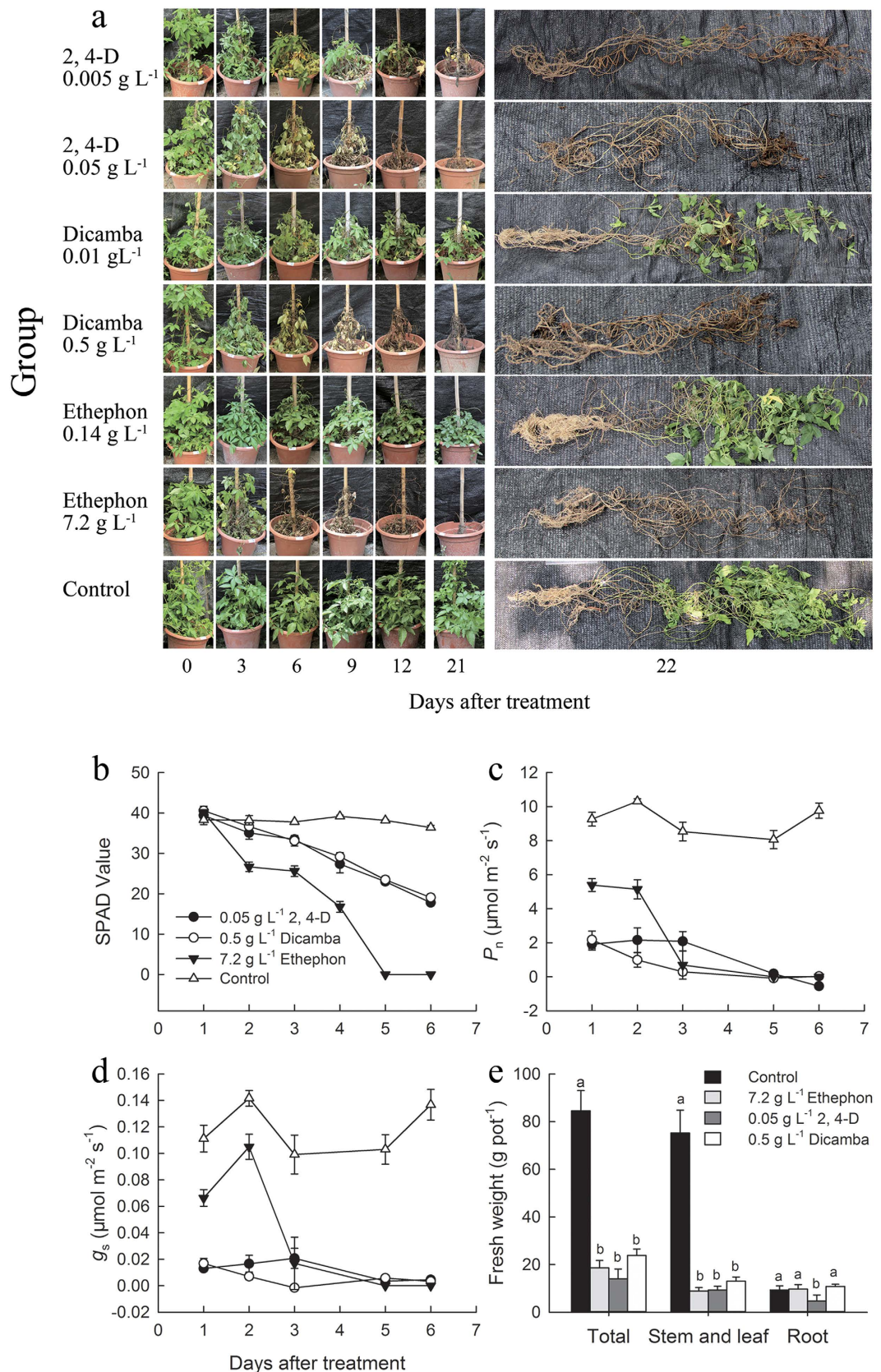
Figure 1. The change in phenotype (a), chlorophyll content (SPAD value, (b), net photosynthesis rate (P n , (c), stomatal conductivity (g s , (d) and fresh weight (e) of Ipomoea cairica in a pot experiment. Data are means ± SE. The columns with different letters are significantly different with each other ( p < 0.05 ).
