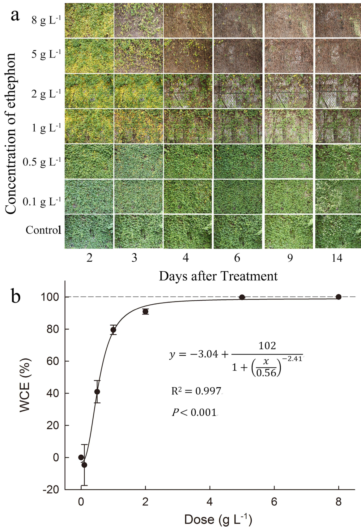
Figure 4. (a). The visual change of Ipomoea cairica treated with a concentration gradient of ethephon in a field experiment; (b). The logistic WCE-dose curve for the use of ethephon to control Ipomoea cairica . Data were means \pm SE.
