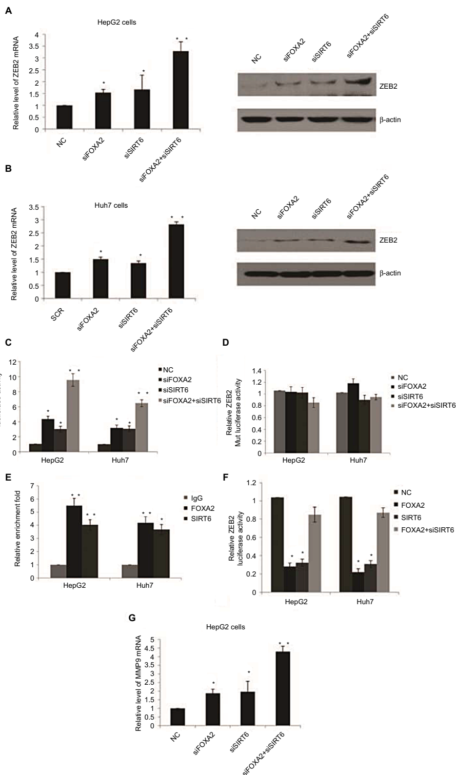
Figure 5 FOXA2 and SIRT6 repress the expression of ZEB2 transcriptionally.
