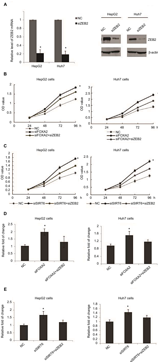
Figure 6 ZEB2 suppression involved in the anti-oncogenesis effect of FOXA2 and SIRT6.
