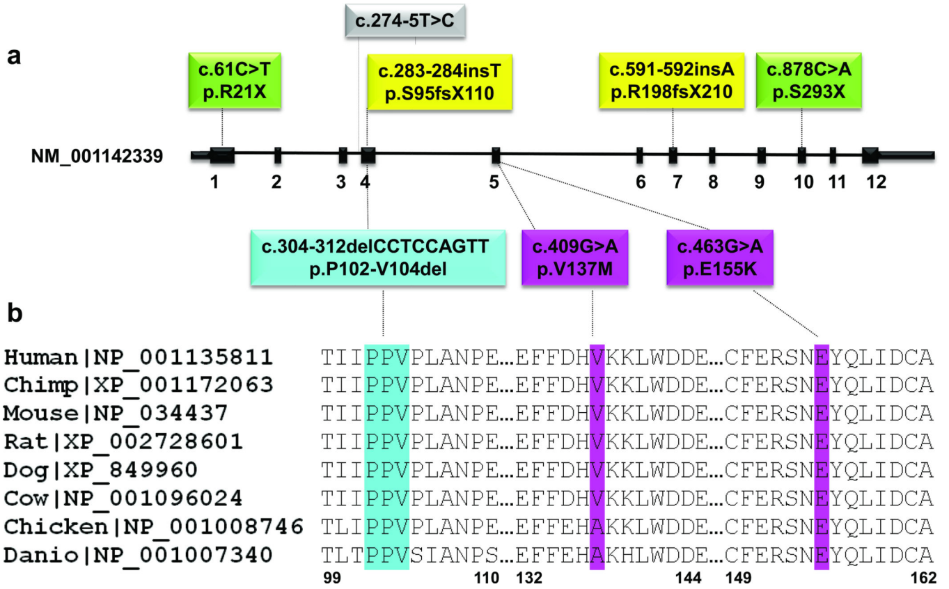
Figure 1. Mutations identified in GNAL in PTD patients. a. Schematic representation of exon:intron structure of the short isoform of GNAL (NM_001142339) with mutations indicated. Missense mutations are depicted in pink, in-frame deletion is in blue, nonsense mutations are in green, frame-shift mutations are in yellow and the tentative splice mutation is in grey. b. Protein sequence alignment of Gaolf orthologs from vertebrate species. Protein sequences were obtained from RefSeq database and aligned using ClustalW 57 . The regions of alignment corresponding to the in-frame deletion and missense mutations are shown. The mutations are colored as in panel a. RefSeq accession numbers are indicated.
