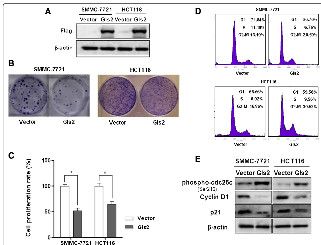
Figure 4 Gls2 suppressed cancer cell growth and induced cell cycle arrest. (A) Ectopic expression of Gls2 in human liver and colon cancer cells. SMMC-7721 and HCT116 cells were transiently transfected with either empty vector or 3 × Flag-tagged Gls2 expressing vector and the expression level of Gls2 was measured by western blot. β-actin served as a loading control. (B) Cell proliferation ability was measured by colony formation assay, which was performed as described in Methods. (C) Overexpression of Gls2 inhibited cancer cell proliferation measured by MTS assay. The values obtained from transfected and control cells represent mean ± SD of three independent experiments. * p < 0.05 between the two groups were calculated using individual Student's t-test. (D) Changes of the cell cycle profiles in cancer cells after Gls2 overexpression were determined using flow cytometry, with representative histograms shown for each treatment. (E) Changes of cell cycle regulators (phospho-cdc25 (Ser216), p21 and cyclin D1) were determined using western blotting. β-actin was used as the internal control.
