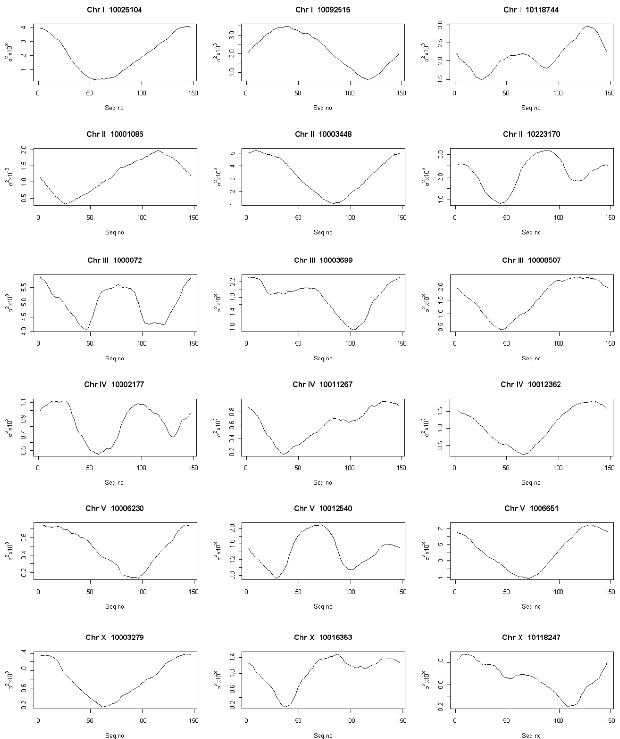
Figure 1 Curvature dispersion Curvature dispersion \sigma^2 associated with C. elegans nucleosome calculated by cyclically permuting the sequences using the theoretical model proposed by De Santis et al [46]. The minima correspond to the molecular bend locus of the fragment.
