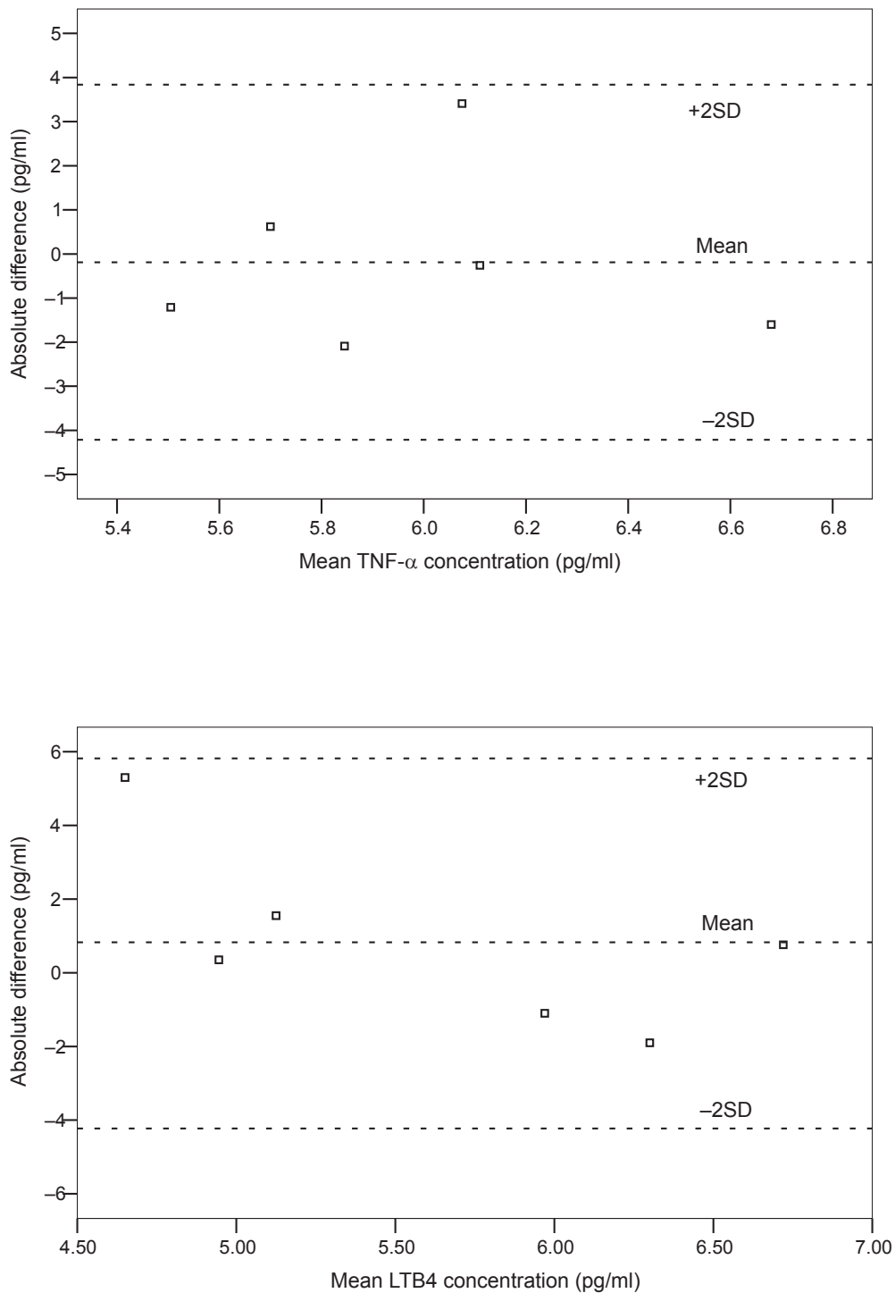
Figure 2 Bland and Altman's plot of the repeatability measurements of TNF- \alpha and LTB4.
