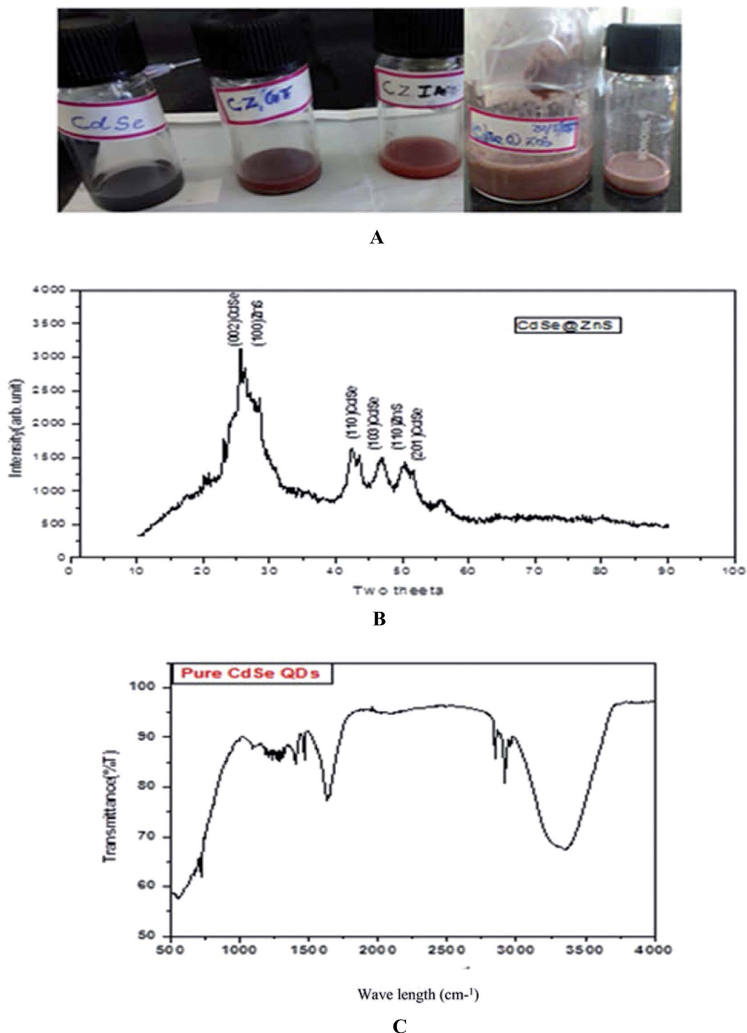
Fig. 1 (A, top) as prepared quantum dot samples. (B, middle) XRD pattern of the CdSe@ZnS sample. (C, bottom) FTIR spectrum of Pure CdSe.
