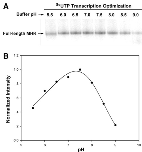
FIGURE 4. Experimental results of transcription optimizations with Se UTP. (A) Optimization of the transcription buffer pH (5.5–9.0). pH 7.5 is optimal for the Se-RNA transcription, while the pH of the standard transcription buffer is 7.9. (B) Data analysis of the pH optimization.
