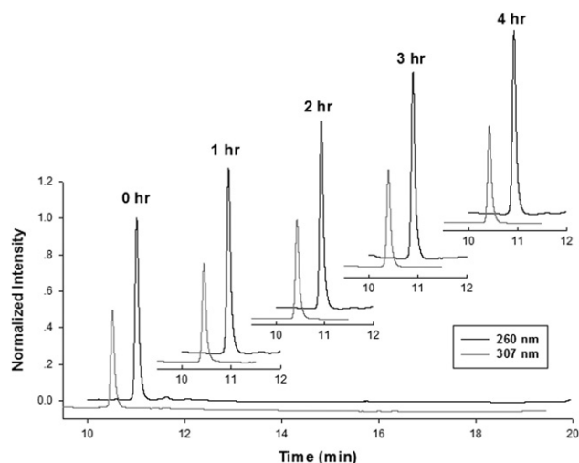
FIGURE 6. Thermostability study of ^{76}\text{SeU} -RNA. 5' \text{-U}^{76}\text{UU-3}' was heated at 70^\circ\text{C} for several hours. HPLC was monitored at both 260 and 307 nm (retention time: 10.9 min).
