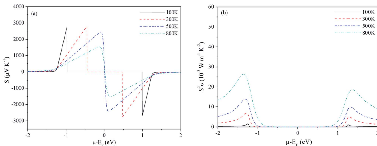
Fig. 2 Variation of (a) Seebeck coefficient and (b) power factor of \text{Be}_2\text{C} with chemical potential at \tau = 4 \times 10^{-14} \text{ s} .
