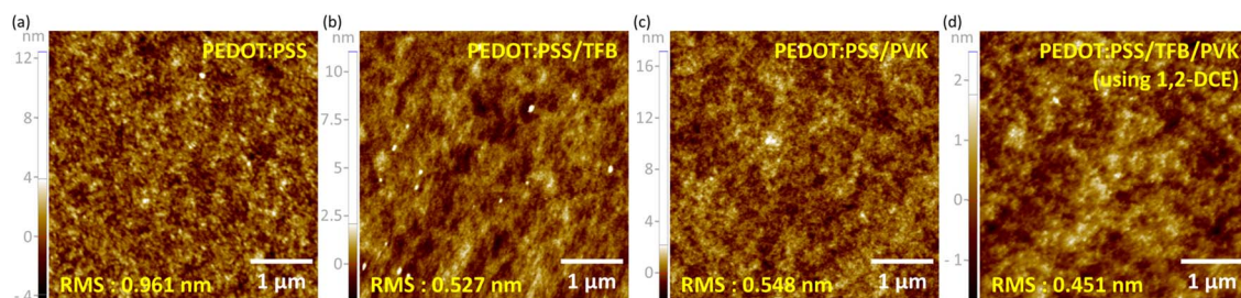
Fig. 2 AFM images (5 \mu\text{m} \times 5 \mu\text{m} ) of (a) PEDOT:PSS, (b) PEDOT:PSS/TFB, (c) PEDOT:PSS/PVK, and (d) PEDOT:PSS/TFB/PVK using 1,2-DCE as the PVK solvent.
