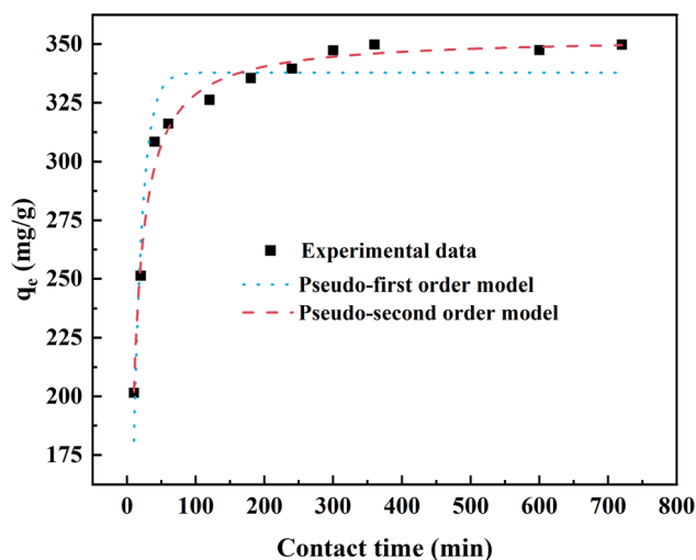
Fig. 6 Kinetic model fitting results for fluoride adsorption by AES900. ( [F^-]_0 = 600 \text{ mg L}^{-1} , [\text{adsorbent}] = 1 \text{ g L}^{-1} , temperature = 20 \text{ }^\circ\text{C} and pH at neutral).
