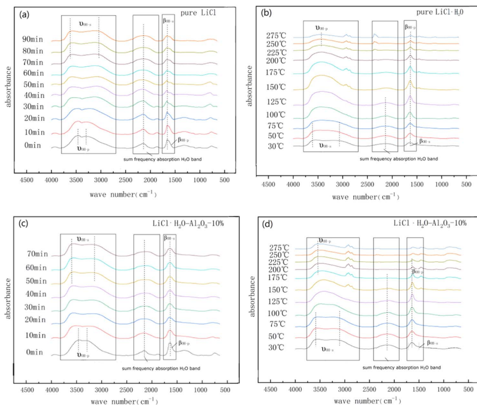
Fig. 4 The in situ DRIFT spectroscopy of (a) the hydration reaction of LiCl; (b) dehydration reaction of \text{LiCl}\cdot\text{H}_2\text{O} ; (c) hydration reaction of \text{LiCl}\cdot\text{H}_2\text{O}\text{-Al}_2\text{O}_3\text{-10\%} ; (d) dehydration reaction of \text{LiCl}\cdot\text{H}_2\text{O}\text{-Al}_2\text{O}_3\text{-10\%} .
