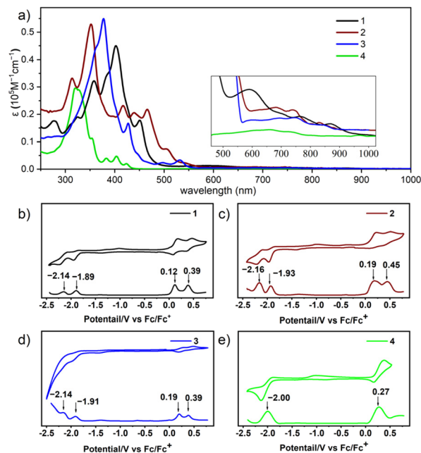
Fig. 4 (a) UV-vis absorption ( 10^{-6} M in DCM). Cyclic voltammetry (CV) curves and differential pulse voltammetry (DPV) curves of (b) 1 , (c) 2 , (d) 3 , and (e) 4 , measured in 0.1 M solution of {}^n\text{Bu}_4\text{NPF}_6 in DCM.
