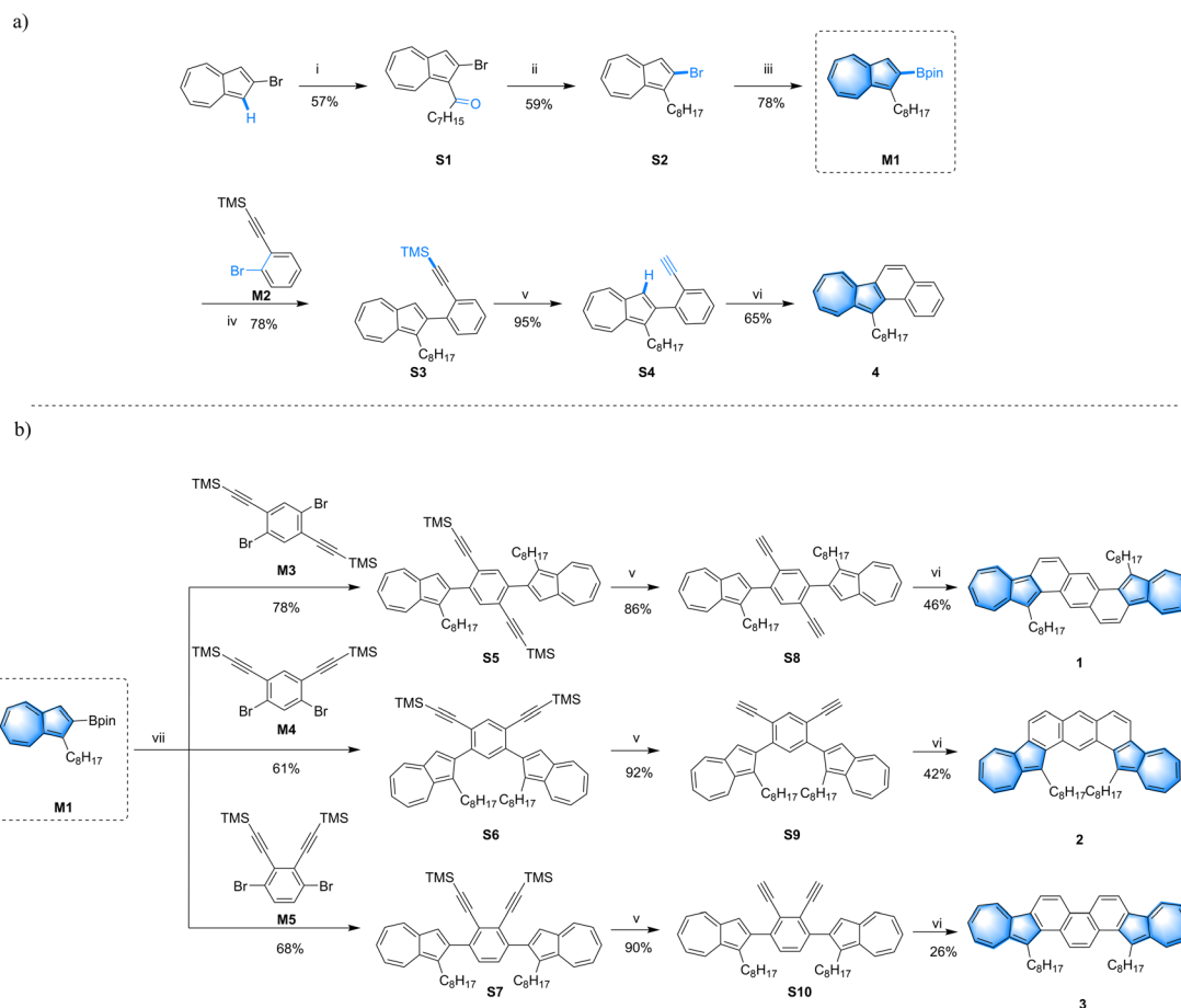
Scheme 1 Chemical structures and synthetic routes of compound 4 (a), and compounds 1–3 (b): (i) \text{AlCl}_3 , octanoyl chloride, DCM, 0\text{ }^\circ\text{C} ; (ii) \text{BH}_3\cdot\text{THF} , \text{BF}_3\cdot\text{Et}_2\text{O} , THF, 0\text{ }^\circ\text{C} to r.t.; (iii) \text{B}_2\text{Pin}_2 , \text{Pd}(\text{dppf})\text{Cl}_2 , KOAc, DMSO, 80\text{ }^\circ\text{C} ; (iv) \text{Pd}(\text{PPh}_3)_4 , \text{K}_2\text{CO}_3 , toluene/EtOH/ \text{H}_2\text{O} , 85\text{ }^\circ\text{C} ; (v) KF, DMF/ \text{H}_2\text{O} , r.t.; (vi) \text{PtCl}_2 , toluene, 85\text{ }^\circ\text{C} ; (vii) \text{Pd}_2(\text{dba})_3 , XPhos, \text{K}_2\text{CO}_3 , THF/ \text{H}_2\text{O} , 85\text{ }^\circ\text{C} .
