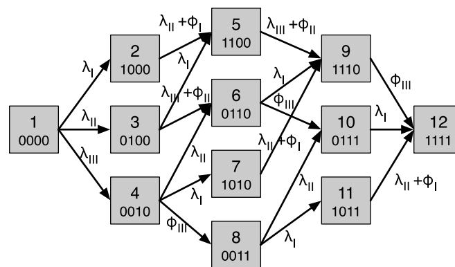
Fig 5. The state transition diagram for the tongue cancer model. Each node corresponds to a possible metastatic state and is represented by a binary string which signifies which lymph node station is positive or negative. For convenience the nodes are named from 1 to 12. The rates are obtained from the flow rates in the anatomic network (Fig 1) by considering the rate at which individual sites become positive based on the state of the other sites.
