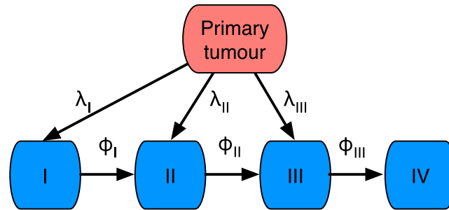
Fig 1. Schematic of the flow of metastatic cells in the case of tongue cancer. The cancer cells flow from the primary tumour to lymph node station I, II and III with rates \lambda_I , \lambda_{II} and \lambda_{III} respectively. The flow between lymph node stations is defined by the rates \phi_I , \phi_{II} and \phi_{III} .
