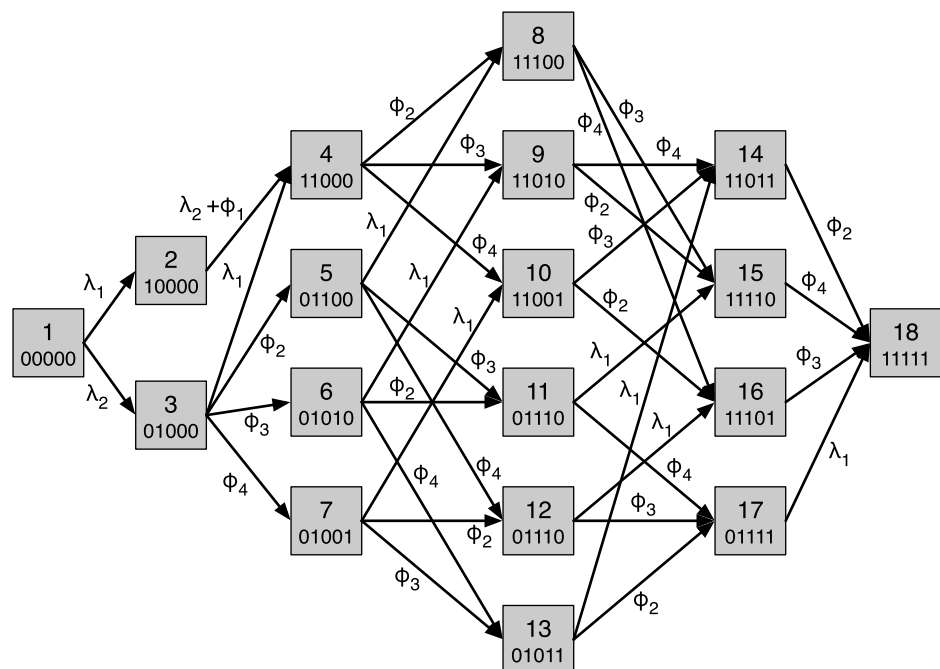
Fig 7. The state transition diagram for the ovarian cancer model. Each node corresponds to a possible metastatic state and is represented by a binary string which signifies which organ is positive or negative for metastases. For convenience the nodes are named from 1 to 18. The rates are obtained from the flow rates in the anatomic network (Fig 3) by considering the rate at which individual sites become positive based on the state of the other sites.
