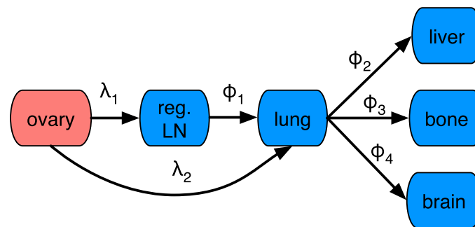
Fig 3. The dissemination network for ovarian cancer. The tumour cells spread either via regional lymph nodes or directly to the lung where they form metastases. From there further dissemination to the liver, bone and brain occurs.
