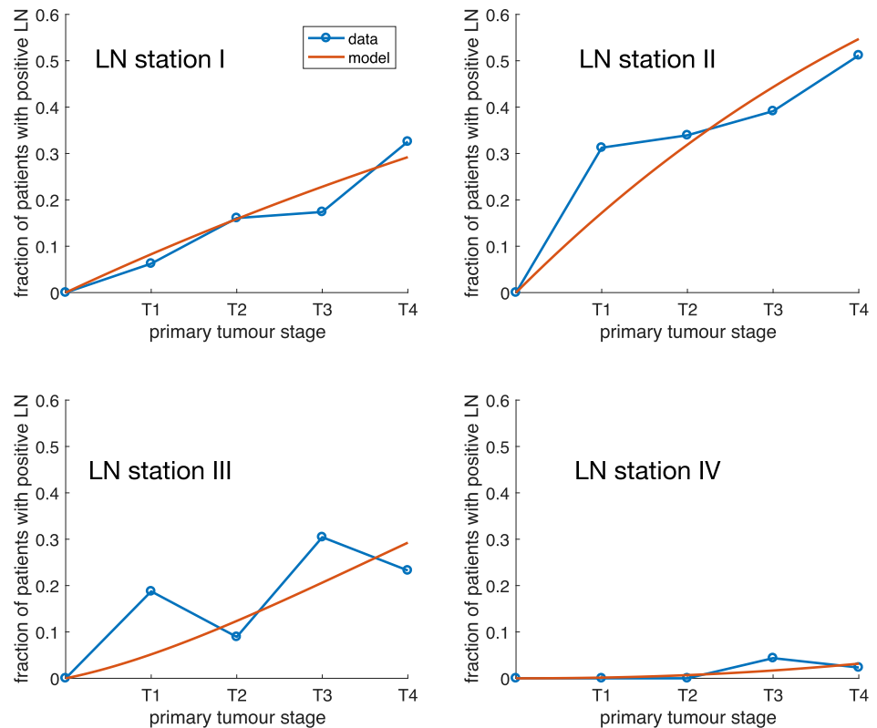
Fig 2. The data and model predictions for metastatic spread to lymph node station I-IV for primary tongue cancer. Each panel corresponds to a lymph node station and shows the probability of finding a metastases in the lymph node as a function of the primary tumour stage. The parameters of the model are given in Table 1.
