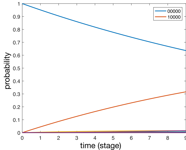
Fig 8. A solution to Eq (4) with parameter values obtained from the maximum likelihood method. Each curve correspond to specific state of the system.
