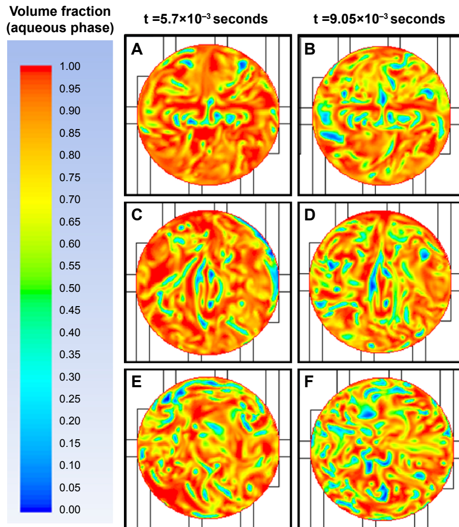
Figure S7 Microchannel emulsification at 24^{\circ}\text{C} .
