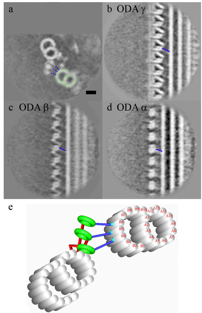
Figure 4. The attachment of the ODA stalk to the adjacent microtubule. (a–d) It is shown as a cross section (a), ODA \gamma (b), ODA \beta (c), and ODA \alpha (d). The dotted blue lines indicate the stalk. The green circles indicate the protofilaments in the adjacent B-tubule. (e) A model of ODA stalk interaction with the adjacent B-tubule is shown. Bar, 20 nm.
