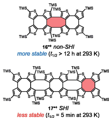
Fig. 14 Chemical structures of thiophene-based double helix radicals 16 and 17 +\cdot (TMS = trimethylsilyl). The molecular fragment in red highlights the predominant localization of the SOMO within the molecular structure.
