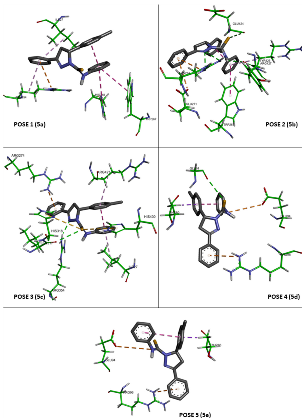
Figure 5. Three-dimensional binding modes of compound 4a (pose 1–5) present at the active sites of CYP51. The interaction modes of the most potent pose in CYP51: Figure 5a orientation 4a in pose 1, Figure 5b orientation 4a in pose 2, Figure 5c orientation 4a in pose 3, Figure 5d orientation 4a in pose 4 and Figure 5e orientation 4a in pose 5. Pi-cation/Pi-anion/attractive charge interactions (orange), Pi-sigma interaction (purple), Pi-sulfur (light brown), conventional hydrogen bond interaction (green), unfavorable interaction (red), Pi-Pi T-shaped interaction (pink).
