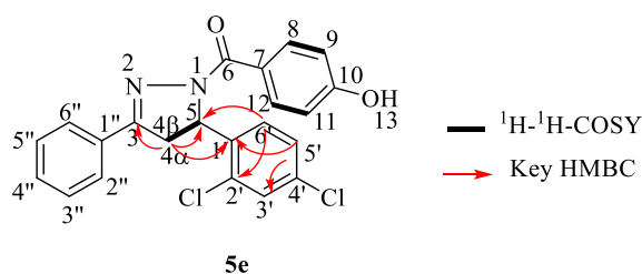
Figure 3. Key COSY/HMBC correlations of compound 5e .
