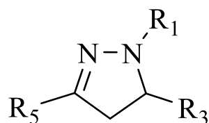
Figure 1. The general structure of the pyrazoline at position 1-, 3- and 5-.
