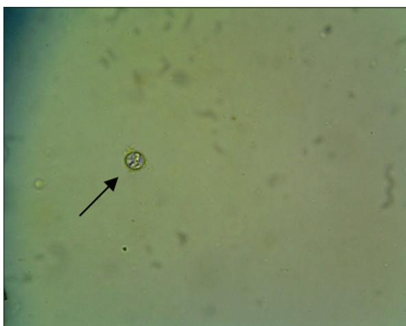
Figure-2: Cryptosporidium spp. (400×).
