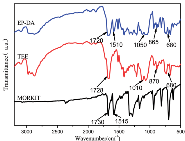
Fig. 2 FTIR spectra of EP-DA, TEE and 1,4-antraquinone.
