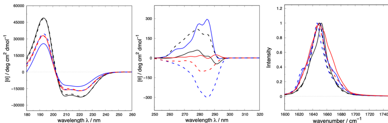
Fig. 3. Calculated spectra of SARS-CoV-2 proteins with models from the Feig group (solid line) or AlphaFold (dashed line). Left: far-UV CD; middle: near-UV CD; right: IR. Colour code: nsp6 (black), M-protein (blue) and nsp4 (red). (For interpretation of the references to colour in this figure legend, the reader is referred to the web version of this article.)
