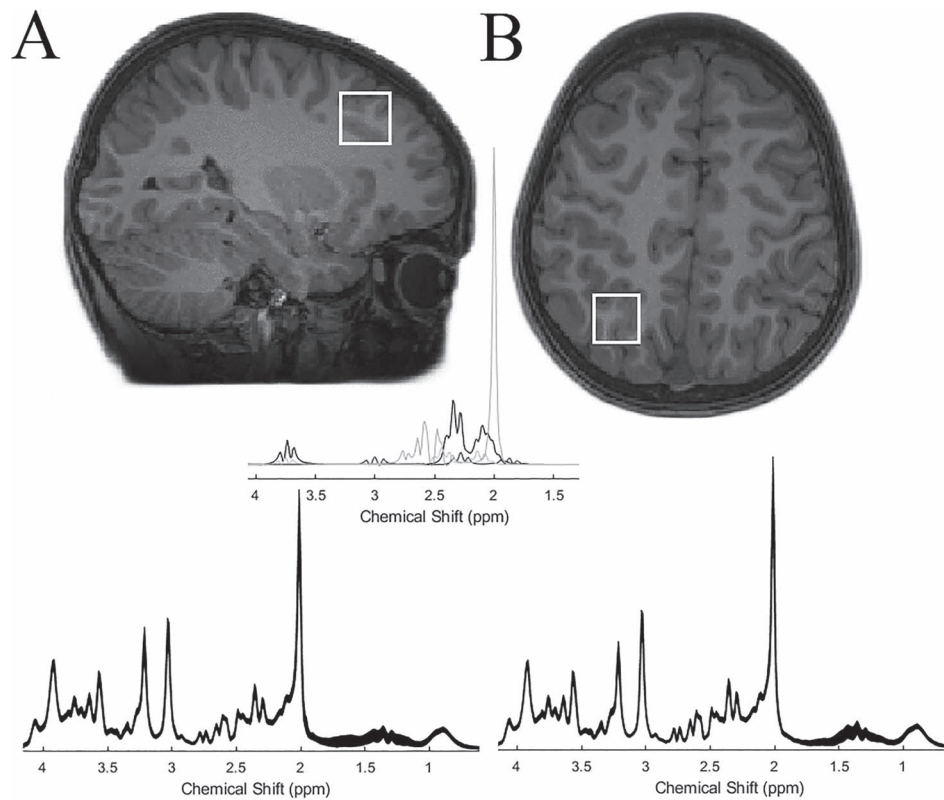
Fig. 1. Positions of the two regions for the MRS displayed in a T1-weighted image for (A) MFG and (B) IPS are shown on sagittal and axial slices, respectively. Below each figure, the mean spectrum from our sample of each region is shown (parts per million, ppm, depicted in x-axis), and the thickness corresponds to \pm 1 SD from the mean. The middle panel shows the fit spectra of glutamate, GABA, glutamine, and N-acetylaspartate.
