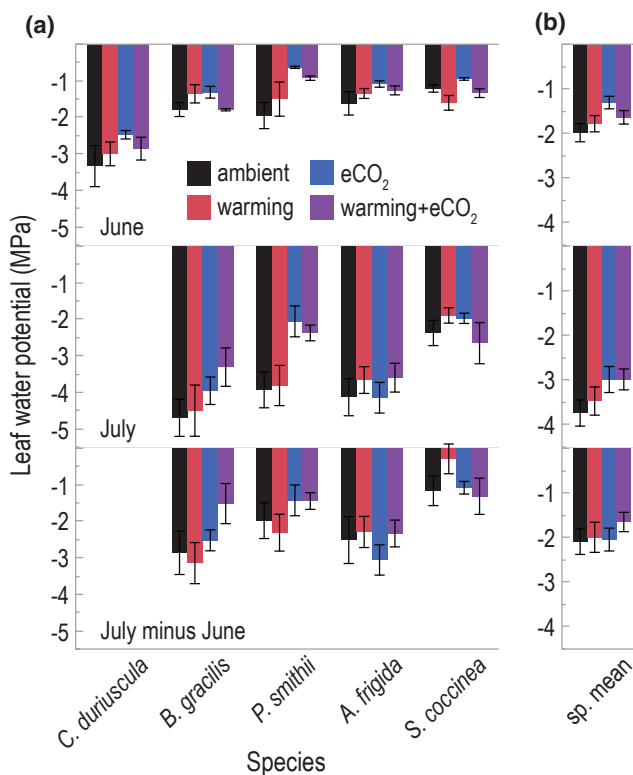
FIGURE 2 Mean leaf water potentials (pre-dawn) for different treatments, species, and sampling periods. The bottom panel shows how much pre-dawn water potentials declined from the first (June) to the second (July) sampling period, mirroring the decline of soil moisture observed in all treatments (Figure 1). The left panel (a) shows treatment means separately for each species, while the right panel (b) shows treatment means averaged across all species. See Table 1 for the modeled effects of species and treatments and their interactions.
