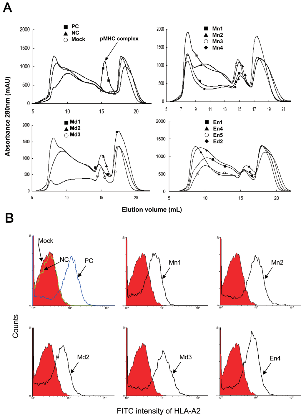
Figure 1. Binding affinity of the synthesized peptides to HLA-A*0201 molecules. A , The refolding results were analyzed by fast-performance liquid chromatography Superdex 200 10/300 GL gel-filtration chromatography, which was calibrated with the standard protein marker, showing that the predicted molecular weight of the protein coming out with 15.2 mL eluting buffer would be 45 kDa, coincident with the molecular mass of the human leukocyte antigen (HLA) complex. A positive control (PC) was performed by the HLA-A*0201-restricted epitope Flu, and the negative control (NC) peptide was CM9 (Table 1). B , In the T2 cell-binding assay, the distribution histograms of cell populations are presented with different fluorescence intensity of fluorescein isothiocyanate (FITC)-anti-HLA-A2 staining of T2 cells cocultured with PC (Flu), NC (CM9), and high-affinity ( FI \geq 1 ) peptides Mn1, Mn2, Md2, Md3, and En4. The results are representative of 3 independent experiments.
