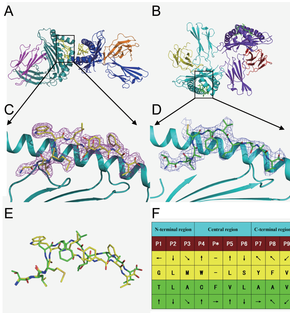
Figure 5. Structures of HLA-A*0201 complexed with Mn2 (GLMWLSYFV) and Md3 (TLACFVLAAV). Structural overviews of HLA-A2 with peptides Mn2 (A) and Md3 (B) demonstrate that both have 2 molecules in 1 asymmetric unit. 2Fo-Fc electron density for Mn2 (C) and Md3 (D) peptides are shown as violet and blue wire (contoured at 1.0 \sigma ) viewed in profile through the HLA-A2 \alpha 2 helix. The carbon atoms are shown as yellow and green for Mn2 and Md3, respectively. E, Comparison of Mn2 (yellow) and Md3 (green) peptide structures by superimposition of the second residues from the N-terminal residues (Leu) and the C-terminal residues (Val). F, General side chain orientation for the 2 peptides as viewed in profile from the peptide N terminus toward the C terminus (up is toward the T cell receptor; down is toward the floor of the peptide binding groove; left is toward the \alpha 1 helix domain; right is toward the \alpha 2 helix domain). The figure was generated using the PyMOL program ( http://www.pymol.org/ ).
