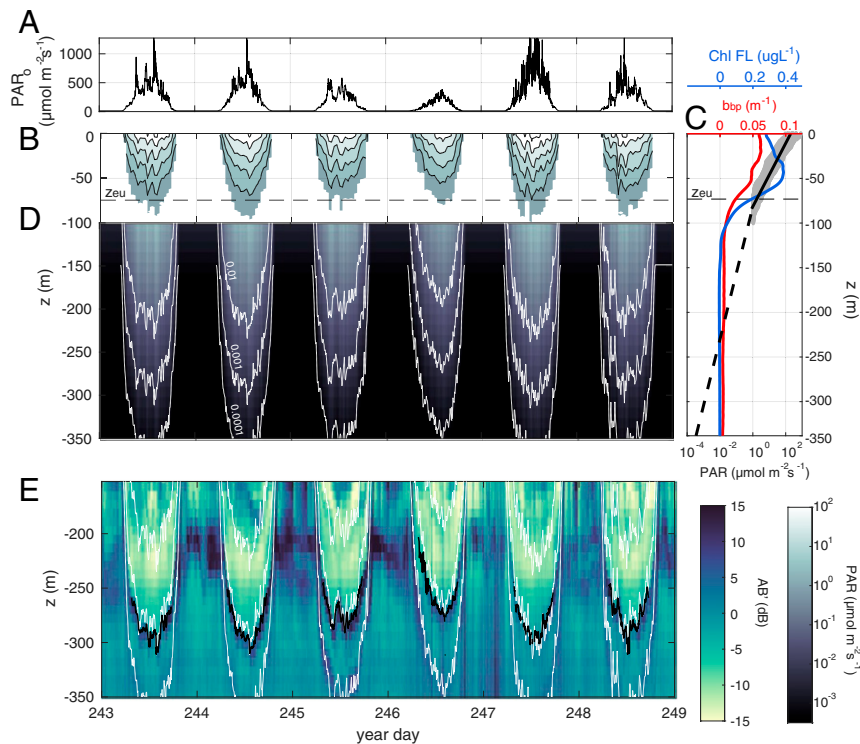
Fig. 1. Time series of (A) surface PAR_o measured from the R/V Reville and (B) PAR depth profile ( PAR_z ) measured from the WW (white space indicates regions where data were removed when the sensor measured below its noise floor of 1 \text{ } \mu\text{mol} \cdot \text{m}^{-2} \cdot \text{s}^{-1} ). (C) WW PAR_z profiles collected between 1000 and 1400 local time (gray points) were fit to estimate the light attenuation coefficient in the euphotic zone, k_{eu} = 0.065 \text{ m}^{-1} , with a 1% light level (horizontal dashed line), z_{eu} , of 71 m occurring just below declines in the average Chl a fluorescence (blue line) and optical backscatter (red line). The average PAR predicted from the twilight zone light attenuation coefficient k_{tz} = 0.03 \text{ m}^{-1} is shown as a dashed black line. (D) Modeled PAR between 100 and 350 m. (E) AB' with isolumes (white contours) and the DSL (black lines). See also SI Appendix , Fig. S2 for the layers evident in the raw AB signal.
