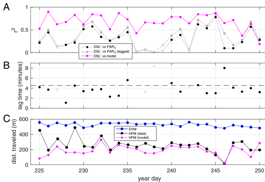
Fig. 3. Daily statistics and distance traveled per day by the migrators. (A) The r^2 correlations between PAR 0 ' and DSL' at zero lag (black dots) and optimal lag (gray dots). Magenta dots indicate the correlation between the high-pass DSL' and the high-pass modeled layer depth anomaly according to Eq. 1. Points with insignificant correlation ( P > 0.001 ) are plotted as open circles. The marked improvement in correlation by the model (even on year days 236–239) occurs because the model captures the lagged response, and smoothes over the most rapid changes in isolume depth. (B) Lag times between PAR 0 ' and DSL' determined by the maximum correlation as indicated on the right-hand column on Fig. 2. (C) Cumulative distance traveled each day during DVM (estimated from AB', blue points) and due to cloud-driven HFM (derived from the DSL' [black] and modeled layer depth [magenta] points). The distance traveled each day due to DVM between the mixed layer (at night) and depth (during day) was calculated from the low-pass-filtered time series from Eq. 2 and the distance traveled due to HFM between 0700 and 1700 each day was estimated by integrating the changes in layer depth.
