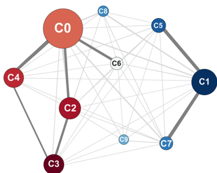
Figure 5. Network plot illustrating population fluxes between clusters 0 and 9. The node radii are proportional to the clusters' equilibrium populations and are positioned using the ForceAtlas algorithm 54 such that states which exchange rapidly are closer to each other. Edge thicknesses are proportional to the fluxes between nodes and fluxes over 25% of the maximum flux, which is between clusters 0 and 4, are highlighted. The nodes are colored according to the cluster mean value of the first nontrivial eigenvector of the MSM transition matrix.
