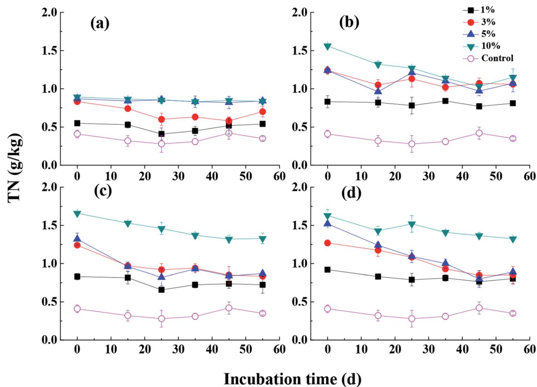
Fig. 4 The effect of MSB produced under different addition of fermentation wastewater on soil TN content ((a) MSB0, (b) MSB1, (c) MSB2, (d) MSB3).
