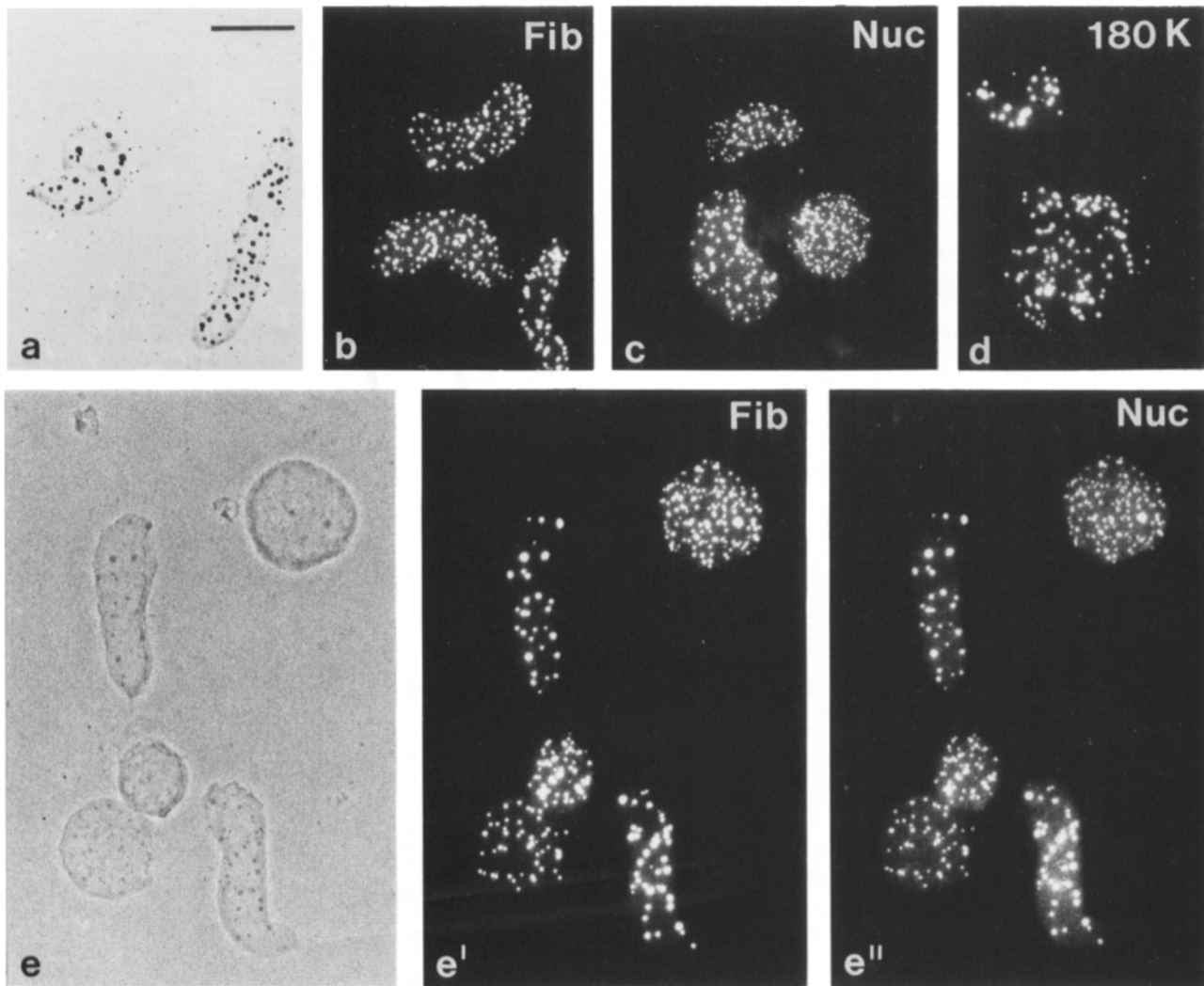
Figure 3. Demembrated sperm nuclei incubated for 90 min in the egg extract and visualized by silver staining ( a ) and immunofluorescence microscopy with antibodies to fibrillar protein ( Fib ; b , e' ), nucleolin ( Nuc ; c , e'' ) and the 180-kD nucleolar protein ( 180K ; d ). Colocalization of the fibrillar protein-containing spots with the antinucleolin staining ( e' , e'' ) is demonstrated by a double-labeling experiment. The larger spots correspond to bodies visible in phase contrast ( e ). Bar, 20 \mu\text{m} .
