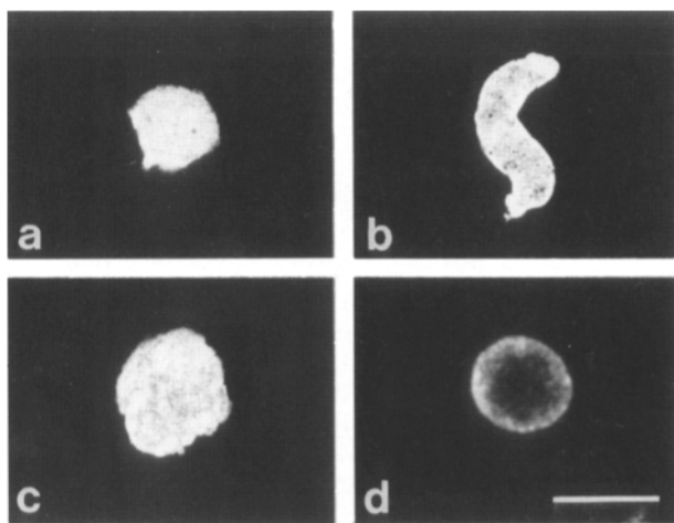
Figure 4. Controls with nonnucleolar antibodies. Nuclei reconstituted from lambda DNA (a, c, d) or sperm chromatin (b) were incubated with antibodies against histones (a, b), DNA (c), and lamina proteins (d) and visualized by immunofluorescence microscopy. In some preparations the dense bodies are clearly visualized as negative dot-like structures within the fluorescent nucleoplasm (e.g., b). Bar, 20 \mu m.
