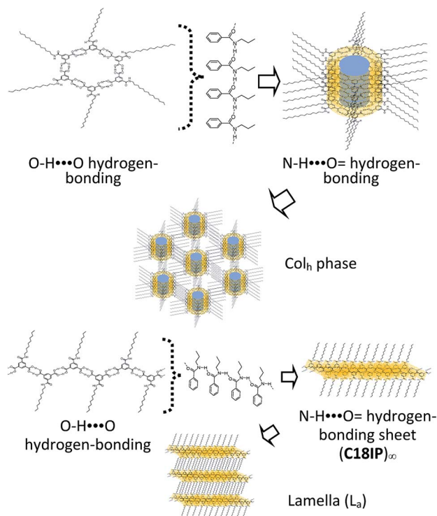
Scheme 3 Formation of the hierarchical molecular assembly structures of C18IP to form the \text{Col}_h (upper) and L_a phases (lower).
