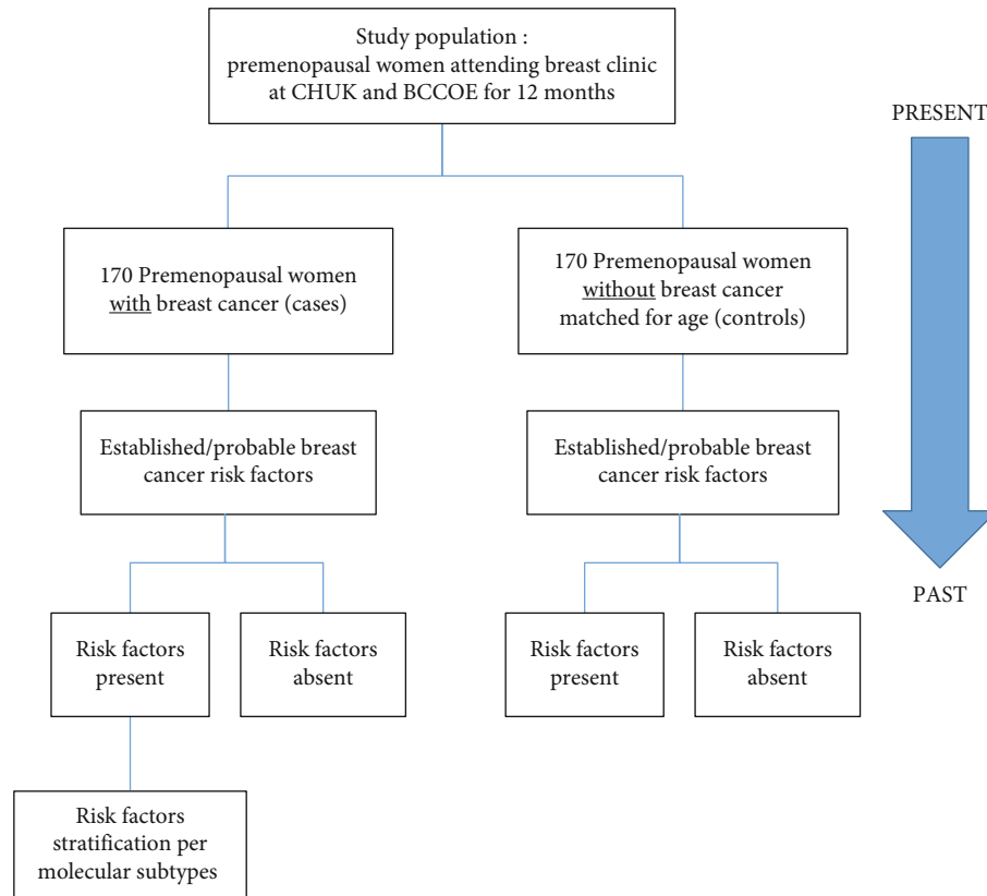
FIGURE 1: Methodology illustration.
