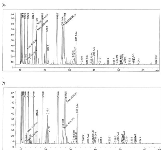
Fig. 2. Fatty acids on samples by gas chromatography with flame ionization detector. (a) butter, (b) cheese.
