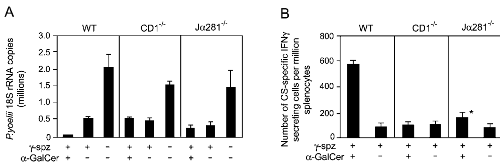
Figure 3. The adjuvant activity of \alpha -GalCer requires CD1d molecules and V \alpha 14 NKT cells. (A) Groups of CD1d-deficient (CD1 -/- ), V \alpha 14 NKT (J \alpha 281 -/- ) deficient and wild-type (WT) mice on a BALB/c background were immunized intravenously with \gamma -spz together with intraperitoneal administration of \alpha -GalCer (+) or vehicle (-). 2 wk later these and nonimmunized mice were challenged with viable sporozoites, and the
