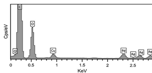
Fig. 2 The EDX spectrum of the Pd/GO nanomaterial.
