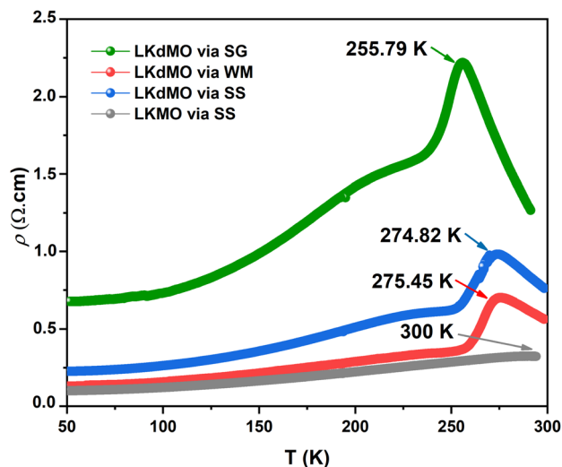
Fig. 13 \rho - T Curves of \text{LKdMO} samples prepared through the SS, WM, and SG methods, and LKMO through SS.
