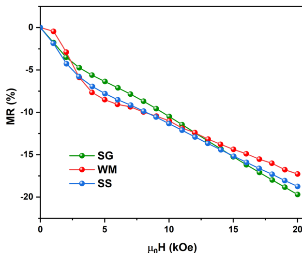
Fig. 15 Field dependence of the MR curve of \text{LK}_d\text{MO} at 150 K.
