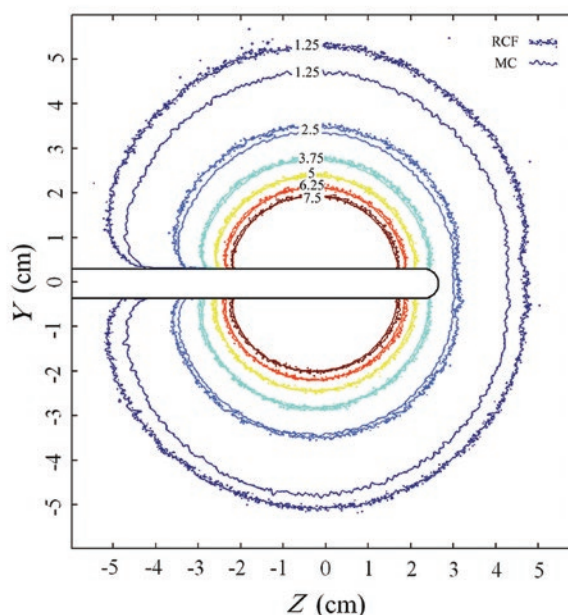
FIGURE 4. Dose distributions (in Gy) for the GZP6 source number one around the tandem applicator in a plane parallel to the long axis of the applicator as obtained by radiochromic films (RCF) measurements and Monte Carlo (MC) simulations.
