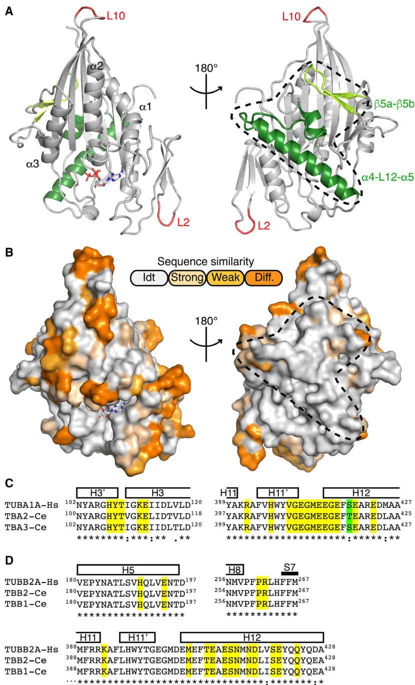
Fig. 5. Human KIF17 motor domain homology model. (A) Representation of KIF17 with the two insertions compared to OSM-3 indicated in red. Two \sim 180^\circ views, centered either on the nucleotide-binding site (left) or on the microtubule-binding surface (delineated by a dashed line; right) are shown. The microtubule-binding elements are colored in green. (B) Surface representation of KIF17 viewed along the same orientations as in the top panel and colored according to sequence conservation compared to OSM-3, as indicated. (C, D) Sequence alignment centered on the kinesin-interacting residues of human \alpha -tubulin (TUBA1A isoform, Uniprot Q71U36 ) with the two most abundant Caenorhabditis elegans \alpha -tubulin isoforms [56] (TBA2, Uniprot P34690 , and TBA3, Uniprot P91910 ; panel C) and of human \beta -tubulin (TUBB2A isoform, Uniprot Q13885 ) with the two most abundant C. elegans \beta -tubulin isoforms [56] (TBB2, Uniprot P52275 , and TBB1, Uniprot O17921 ; panel D). Tubulin residues that are < 5 \text{ \AA} distant from kinesin residues in the tubulin-kinesin-1 complex [8,14] are highlighted in yellow (identical residues) or in green (semi-conserved residues).
