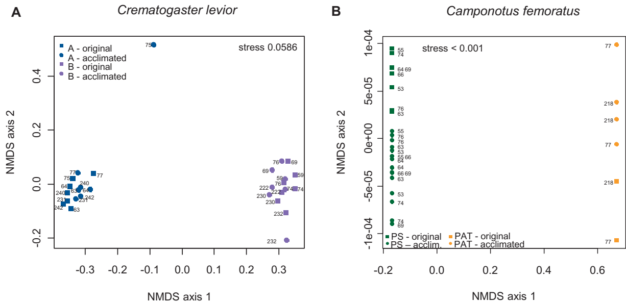
Figure 4 Nonmetric multidimensional scaling (NMDS) of the cuticular hydrocarbon profiles of acclimated and nonacclimated parabiotic ants. Here, we compare the CHC profiles of the cryptic species of (A) Cr. levior and (B) Ca. femoratus from their natural habitat and after 16 days of standardized lab conditions. Each dot represents the CHC profile of one colony. For Ca. femoratus , we had two acclimated individuals per colony but only one extract for the field-collected CHCs. Note that in (A) acclimated sample 075-PAR, albeit aberrant, is clearly Cr. levior A. Cr. levior A is characterized by high abundances of alkadienes with the chain lengths 33, 35, 37, and 39. The relative abundances of these four alkadienes vary across colonies. Here, sample 075-PAR differs from the others in having more C33-dienes and C35-dienes. Also, note that the nearly identical NMDS 1 scores in (B) within each cryptic species stem from the fact that most of the variation is explained by the dichotomous difference between Ca. femoratus PAT and PS.
