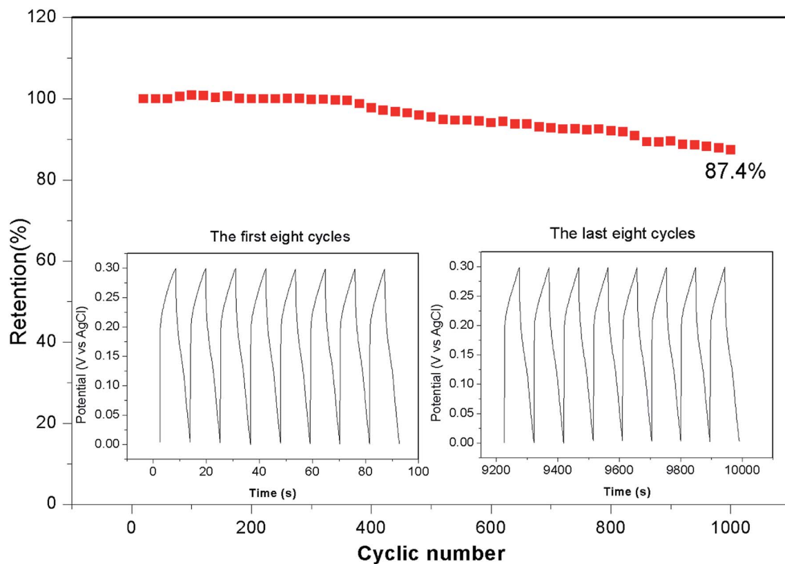
Fig. 6 Cycle performance of Ni-Co-S@ggraphene at a current density of 17 A g^{-1} .
