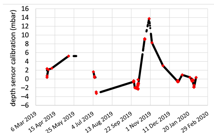
Figure A2. Depth sensor calibration coefficients throughout the monitoring period; red dot—Automatic sensor re-calibration when the HACH probe at its lowest detection limit 9 mm; black dashed line—The linear interpolated calibration coefficient between two automatically generated calibration point; the calibration coefficient is assumed to be constant for the period before the sensor dead.
