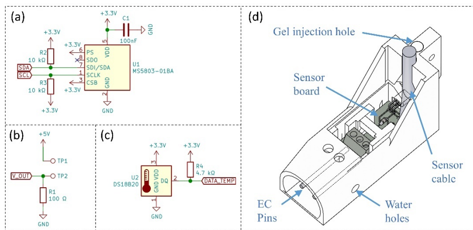
Figure 1. (a) The circuit design of MS5803-01BA sensor with I 2 C communication: +3.3 V for the power supply, GND for ground connection, and SDA and SCL for the I 2 C bus; (b) a simple voltage divider circuit to measure the conductivity of water-based on 5 V power supply: R1 is the selected 100 Ω resistor in this study, TP1 and TP2 are the two screw terminals on the PCB circuit to connect with the stainless steel rod, and V_OUT connects to one of the analog pins on the MCU to measure the voltage drop across R1; (c) the circuit diagram of a digital temperature sensor DS18B20: DATA_TEMP wire connects to one of the digital pins on the MCU to measure the environment temperature; and (d) sensor housing design with a vertical wall at the back of the sensor for easier installation.
