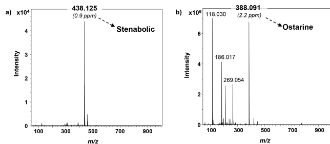
Figure 4. LDTD-ESI–HRMS full-scan spectrum obtained from samples 1 (a) and 10 (b), containing stenabolic and ostarine, respectively.
