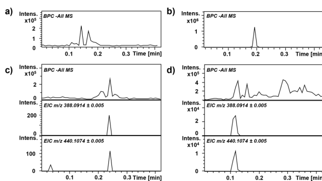
Figure 2. Chronograms obtained by LDTD-ESI–HRMS: base peak chronogram of a blank with (a) white PTFE substrate and (b) black PTFE substrate and extracted ion chronogram of SARMs ostarine and andarine spotted onto (c) white PTFE substrate and (d) black PTFE substrate.
