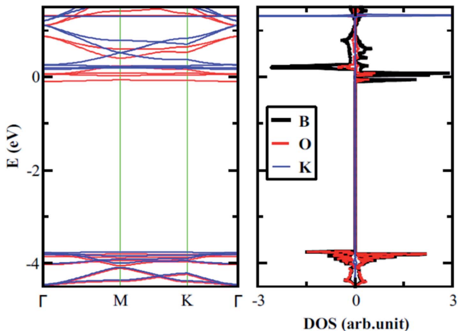
Fig. 8 Band structure and density of states determined for boroxine with a potassium atom adsorbed in the central hole, at the VDW-DF/DZP level of theory.
