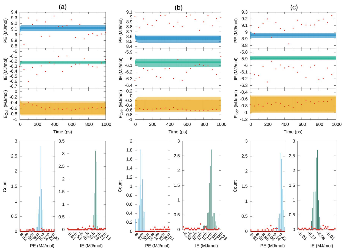
Fig. 8 Forecast prediction of PE and IE for a time span of 1 ns for series in ensemble 100 (top) and the distribution of reported PE and IE values (bottom). The E_{coh} is estimated from the forecasted energetics, eqn (1), and \Delta E mean during the 4–5 ns MD trajectory time predicted in Table 1. (a) Set 1. (b) set 2 and (c) set 3. The dark shaded region denotes forecasted energies from GRU models without cluster-seeding. Light shaded area denotes forecast energies from GRU models with cluster-seeding. Normalization of the histograms is with respect to 70 × 50 000 evaluated time points. Red dots are true energies from a posterior MD simulation for each set.
