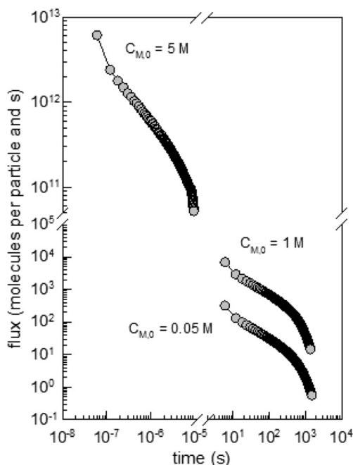
Fig. 4 Correlation between the flux of a swelling agent and the swelling time in a latex particle with a diameter of 100 nm for three different equilibrium concentrations as indicated ( C_{M,0} = 5, 1, and 0.05 M)
