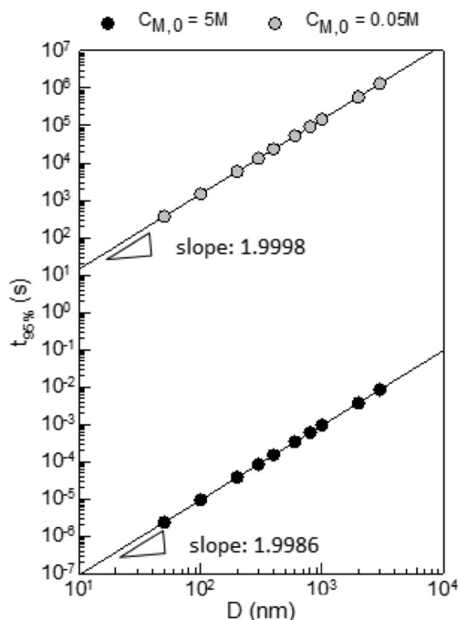
Fig. 3 Correlation between the time it takes to swell a particle to 95% of its equilibrium value ( t_{95\%} ) and the particle diameter ( D ) for two equilibrium concentrations ( C_{M,0} = 5 and 0.05 M) as indicated
