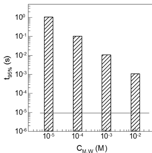
Fig. 7 Correlation between the solubility of the monomer in water ( C_{M,W} ) and the time to reach particle swelling of 95% (for an equilibrium value of C_{M,P} = 5 M) according to the scenario as sketched in Fig. 6 for a particle with 100 nm in diameter which is 150 nm away from the monomer surface ( z = 3 ); the line marks the time which was obtained for such a particle in direct contact with the monomer (cf. Figure 2)
