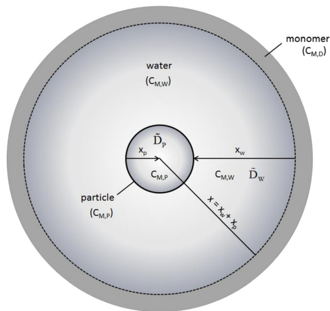
Fig. 6 Sketch of the simulation scenario for diffusion of the swelling agent from a source to the particle through the aqueous phase; the particle is placed in the center of a spherical water layer of thickness x_w which is homogeneously surrounded by a pure swelling agent; for completely penetrating the particle, the swelling agent has to cover the whole distance x = x_w + x_p ; the arrows indicate the final overall direction of the flux of the swelling agent; C_{M,D} , C_{M,W} , and C_{M,P} are the concentrations of the monomer in the source, the water, and the particle, respectively; \tilde{D}_w and \tilde{D}_p are the diffusion coefficients of the monomer in the water and the particle phase, respectively (note, the latter depends on the fraction of the swelling agent inside the particle)
