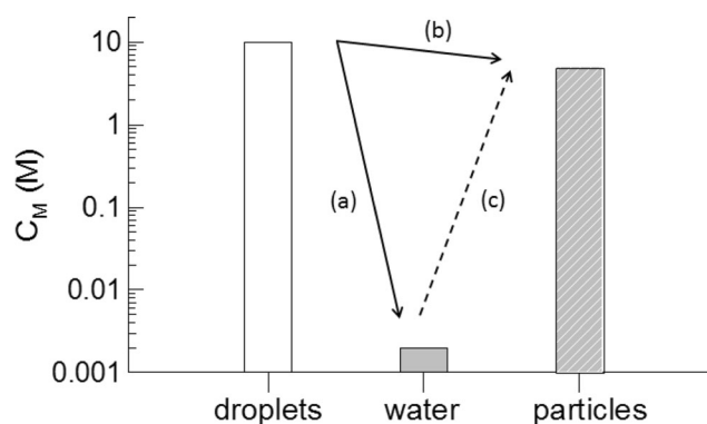
Fig. 1 Distribution of the monomer concentration within the components of a batch emulsion polymerization and illustration of possible diffusion paths: a from the droplets to the aqueous phase, b from the droplets to the particles, and c from the aqueous phase to the particles; the monomer concentration at the various loci are illustrated by the values in a typical range which is in the molar range for droplets and particles (in relation to their corresponding volume) but in the millimolar range for the swelling agent or monomer (such as styrene [18, 19]) in water
