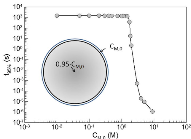
Fig. 2 Correlation between the time it takes to swell a particle (diameter 100 nm) to 95% of its equilibrium value ( t_{95\%} ) and the concentration of the swelling agent in direct contact with particles surface ( C_{M,0} ); the inset sketches are the assumed scenario when the polymerization was stopped; the dots are the simulation results and the line is just for guiding the eyes; the swelling agent is supposed to be located with the concentration C_{M,0} inside an infinitely thin layer as indicated by the bright ring around the particle
