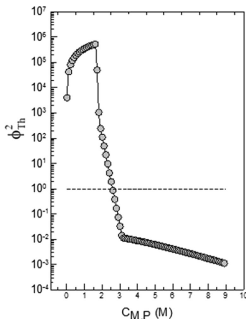
Fig. 5 Correlation of the Thiele modulus with the monomer concentration inside a 100-nm particle ( C_{M,P} ) containing one polymerizing radical; the calculation was made with Eq. 10 assuming an equilibrium situation with respect to C_{M,P} at the particle interface and inside
