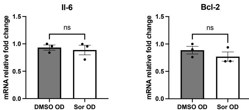
Figure S1. Sorbinil treatment, in the absence of ONC, does not cause changes to inflammation related genes. (A) Fold change expression of il-6 between DMSO and Sorbinil treated retina 1 week after treatment. (B) Fold change expression of bcl-2 between DMSO and Sorbinil treated retina 1 week after treatment.
